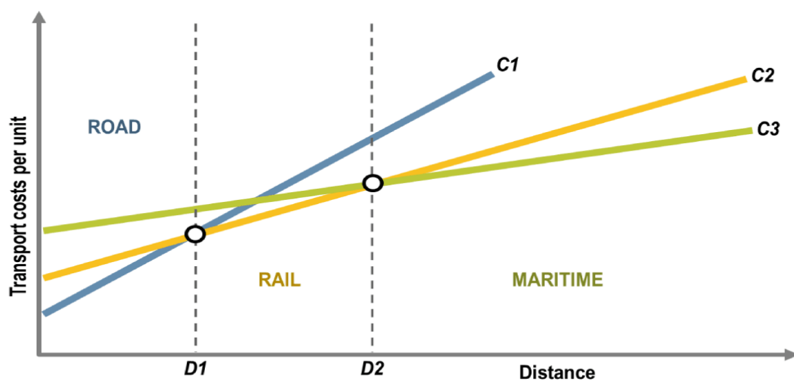
Figure 2 - Generalized comparative cost functions of road (C1), rail (C2) and maritime (C3) transport as a function of distance.
